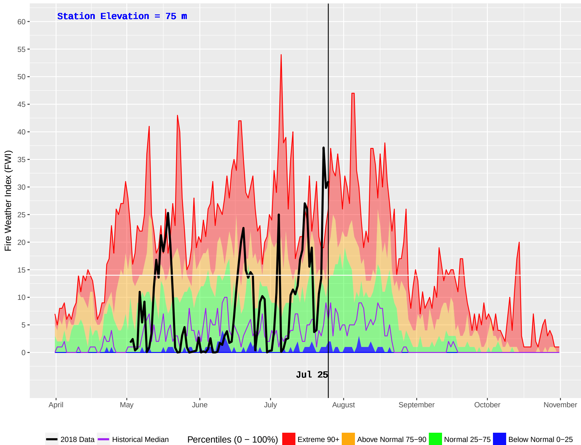
KITPARK (106) : Historical (1995–2016) and Current (2018) Noon Fire Weather Index (FWI)
